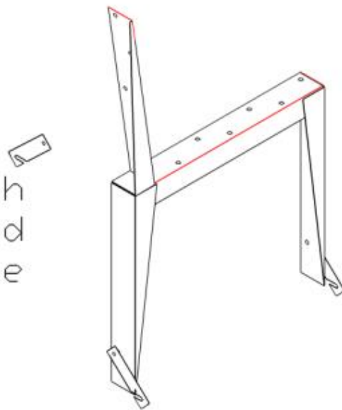
Moveable Bench Frame (Left & Right)
